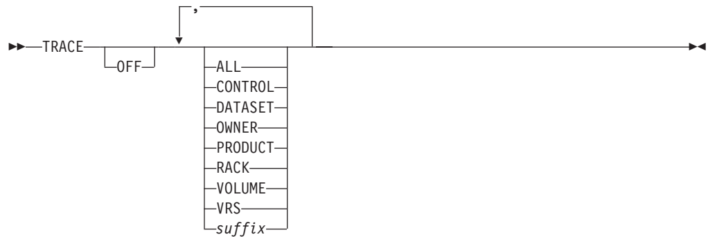
Figure 5. TRACE Command Syntax Diagram
