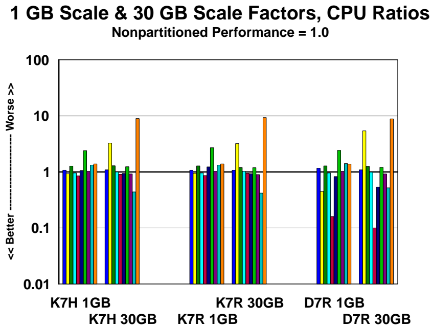
Figure 4.11 CPU time ratios for various Partitioning Schemes Comparing DB Scale Factor s
