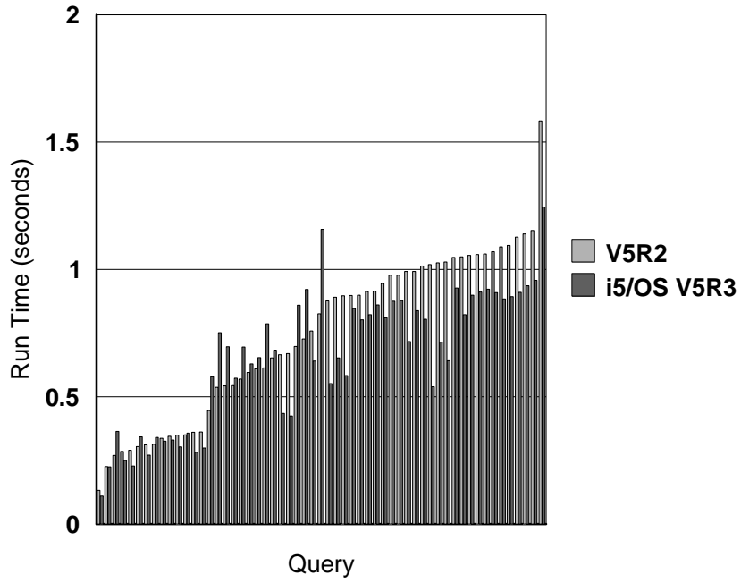
Figure 4.1 Runtime comparison for short running queries (less than 2 seconds)
