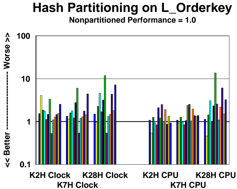
Figure 4.7 Elapsed & CPU time ratios for Hashed Partitioning on L_ORDERKEY
