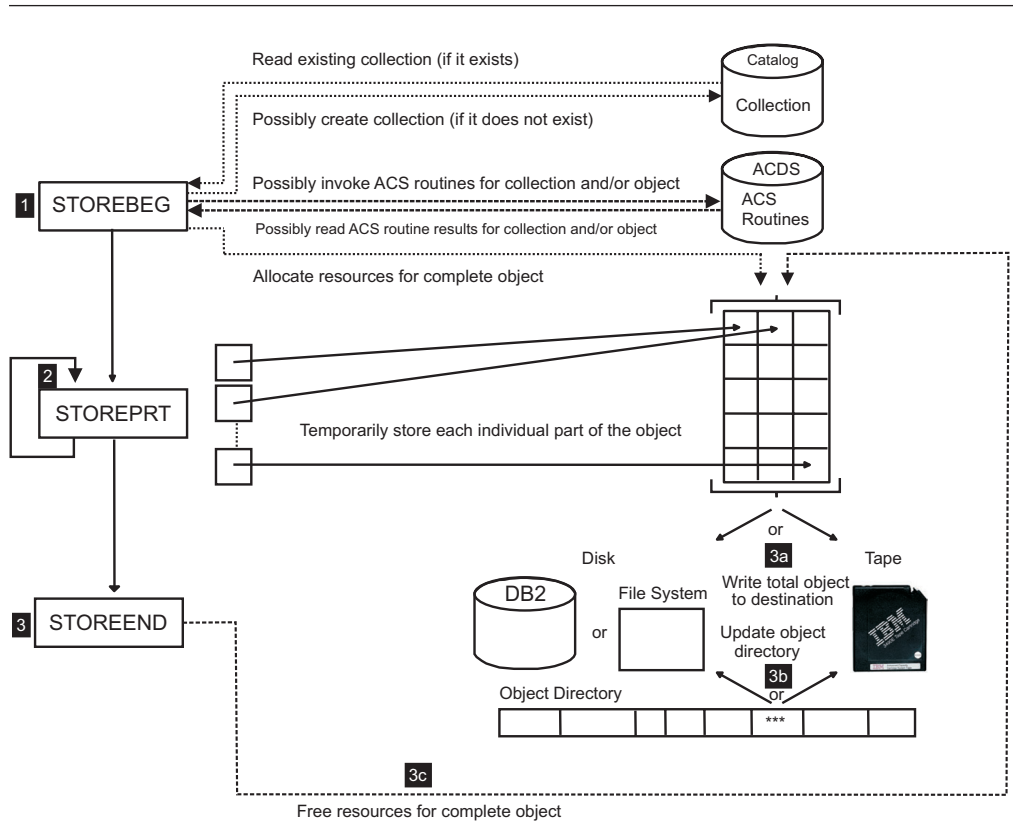
Figure 2. Conceptual View of Storage of Objects Greater Than 256M
