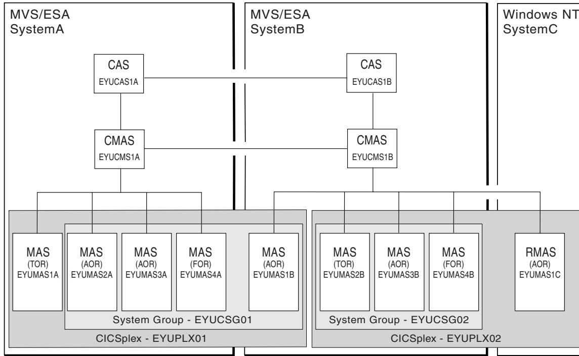
Figure 1. The components of a CICSPlex SM environment
