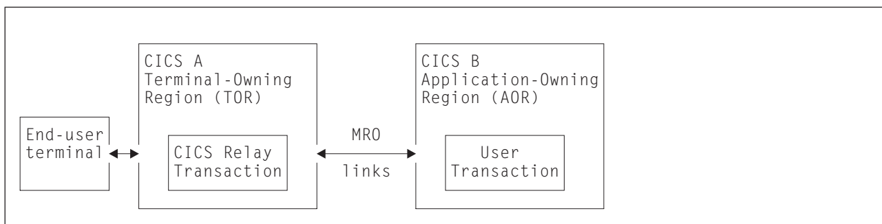
Figure 1. The CICS transaction routing facility
