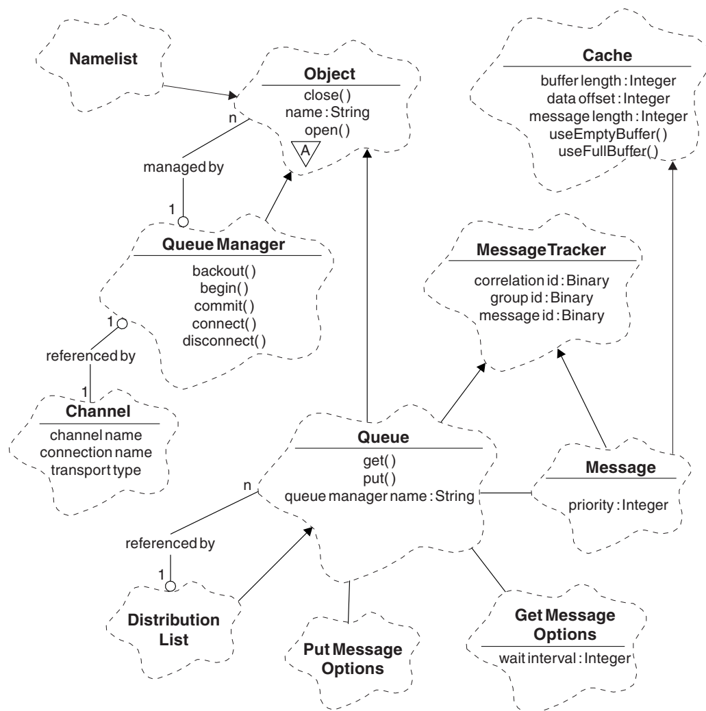
Figure 1. MQSeries C++ classes (queue management)
