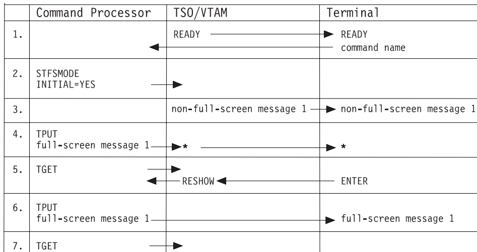
Figure 13. Function of INITIAL=YES when First Message is Non-Full-Screen, Example 1
