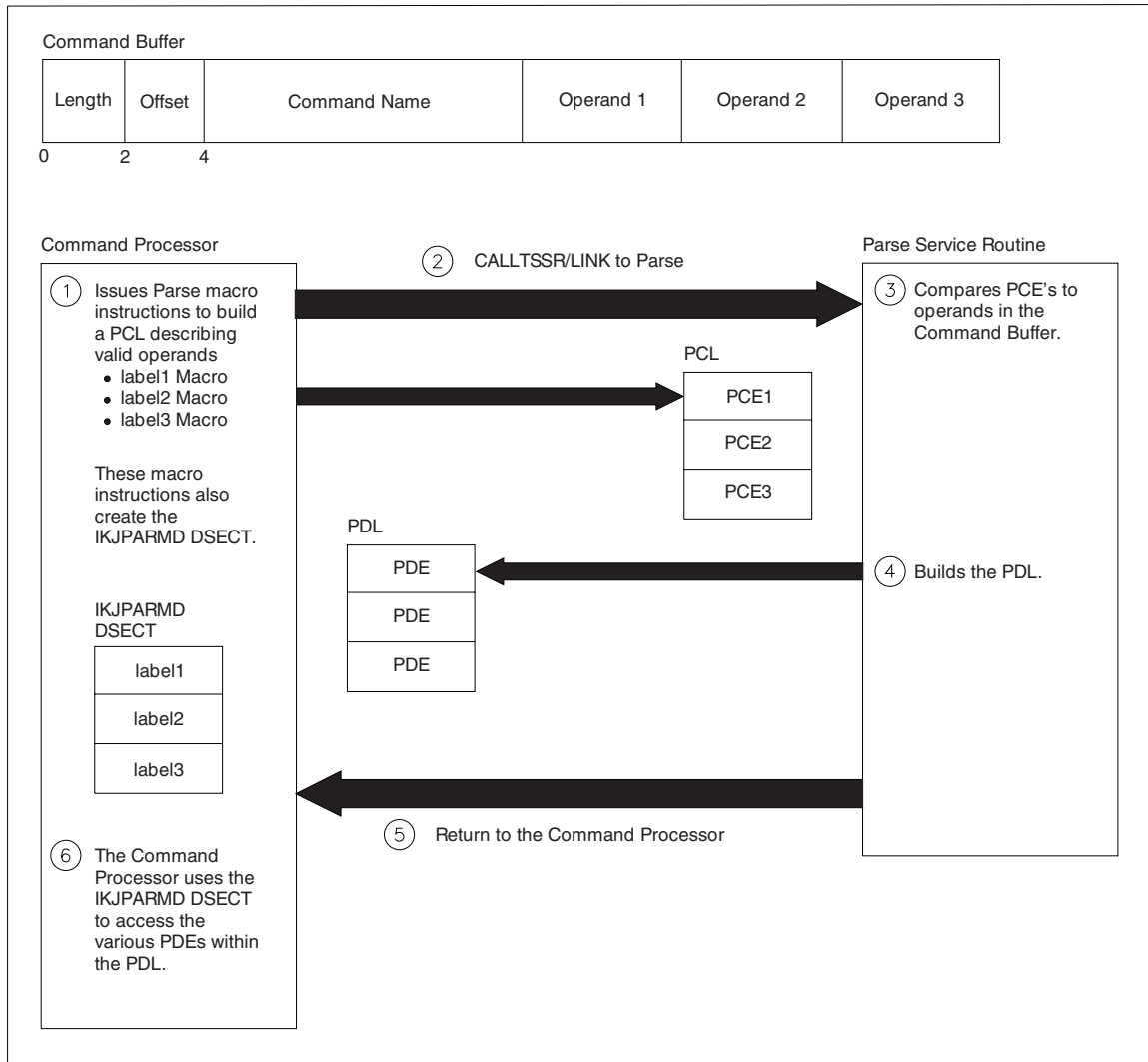
Figure 8. A Command Processor Using the Parse Service Routine
