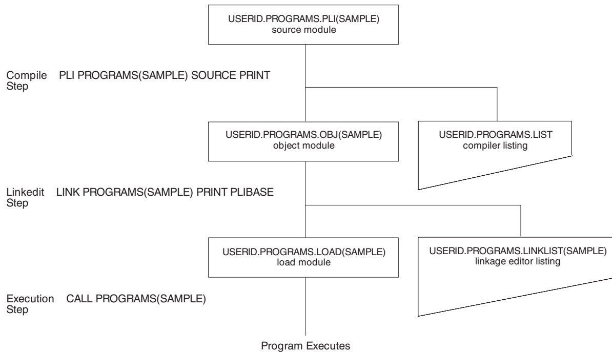
Figure 27. Compiling and Link-Editing a Single Program
