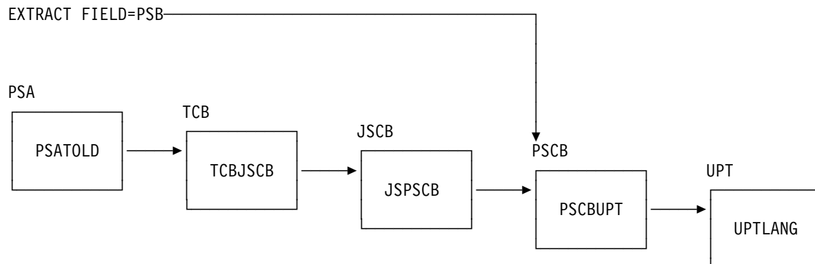
Figure 6. Chaining of Control Blocks and Fields to the UPT
