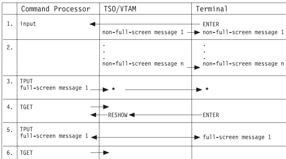
Figure 11. Function of RESHOW in Full-Screen Message Processing
