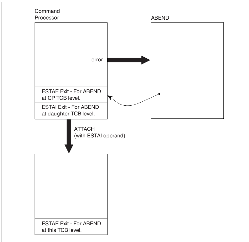
Figure 17. ABEND, ESTAI, ESTAE Relationship
