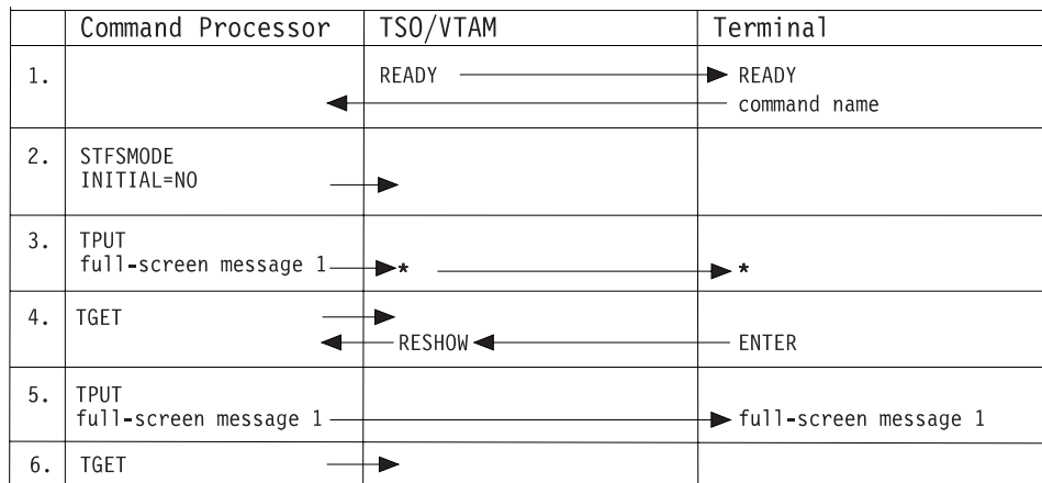
Figure 15. Function of INITIAL=NO
