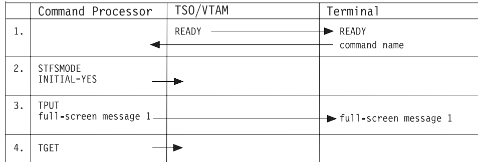
Figure 12. Function of INITIAL=YES when First Message is Full-Screen
