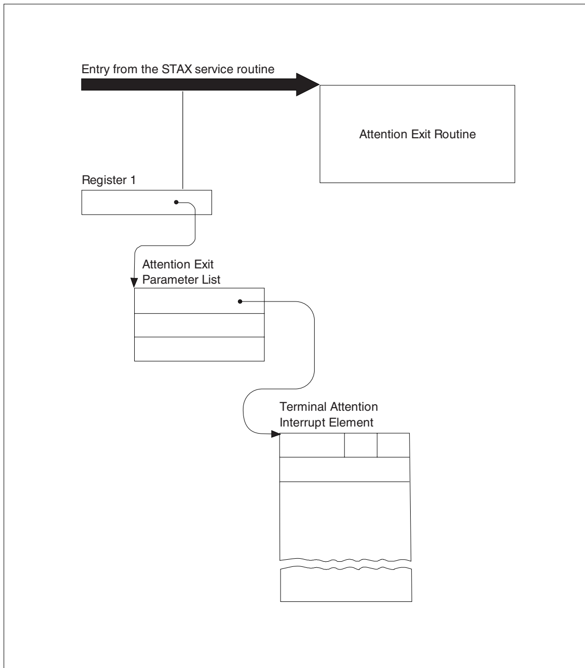
Figure 18. Parameters Passed to the Attention Exit Routine
