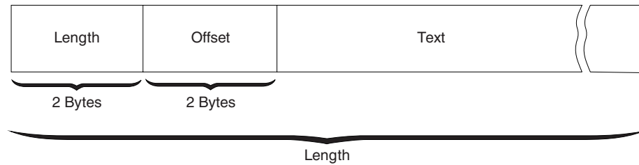
Figure 5. Format of the Command Buffer
