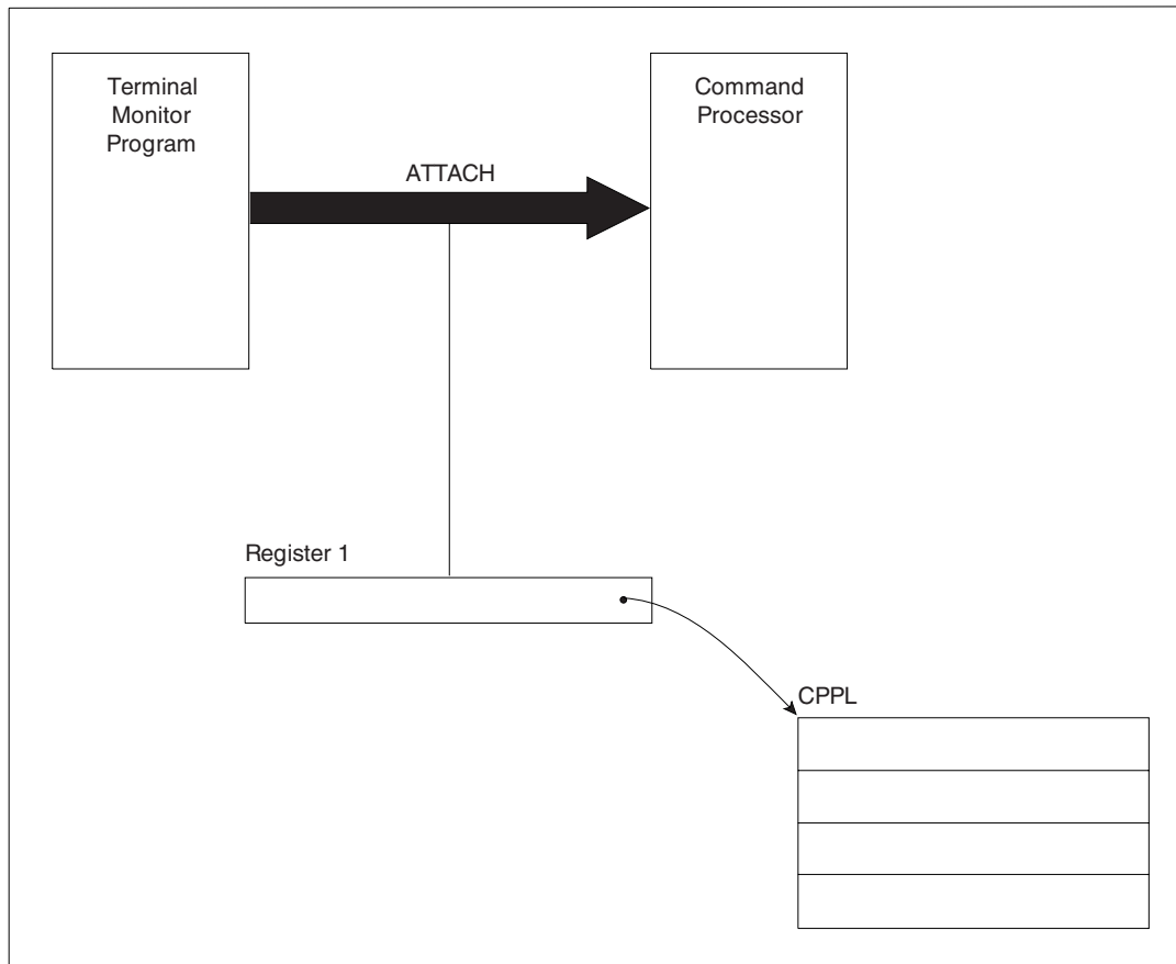
Figure 3. Interface between the TMP and a Command Processor
