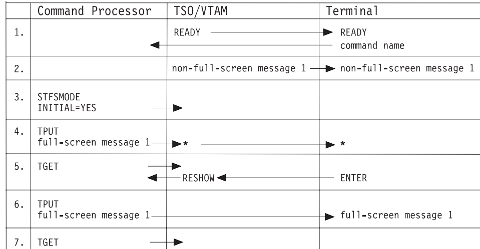
Figure 14. Function of INITIAL=YES when First Message is Non-Full-Screen, Example 2
