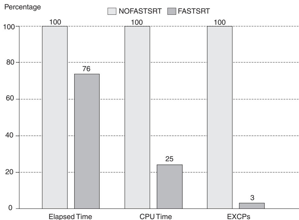
Figure 9. Benefits of FASTSRT
