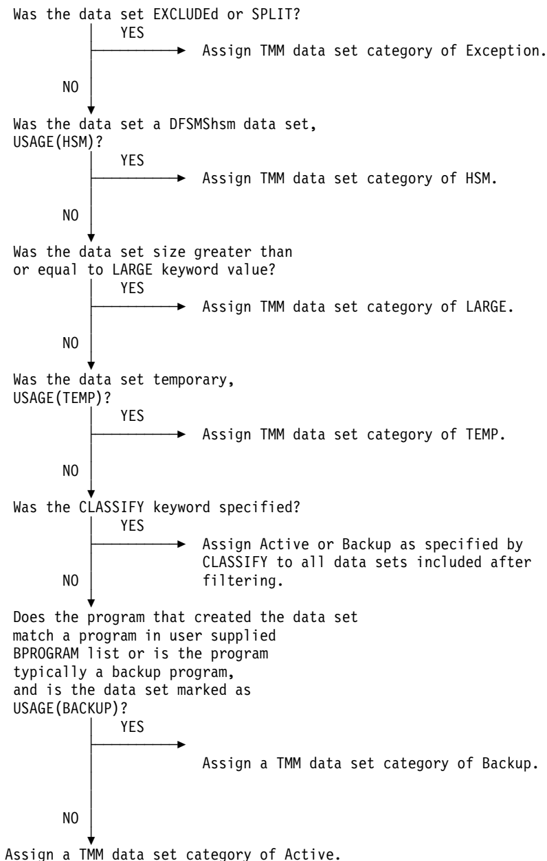
Figure 14. Order of Assigning Tape Mount Management Categories
