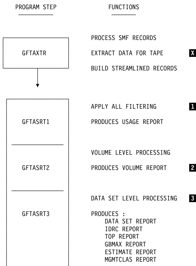
Figure 15. The Three Phases of GFTAVMA Processing
