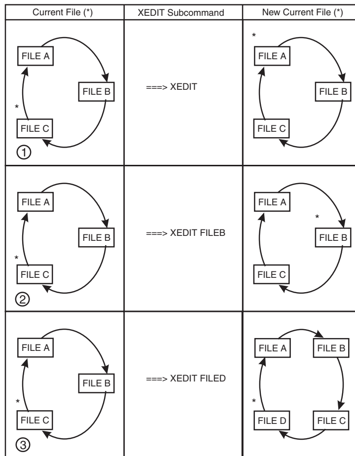
Figure 29. Editing Files in the Ring
