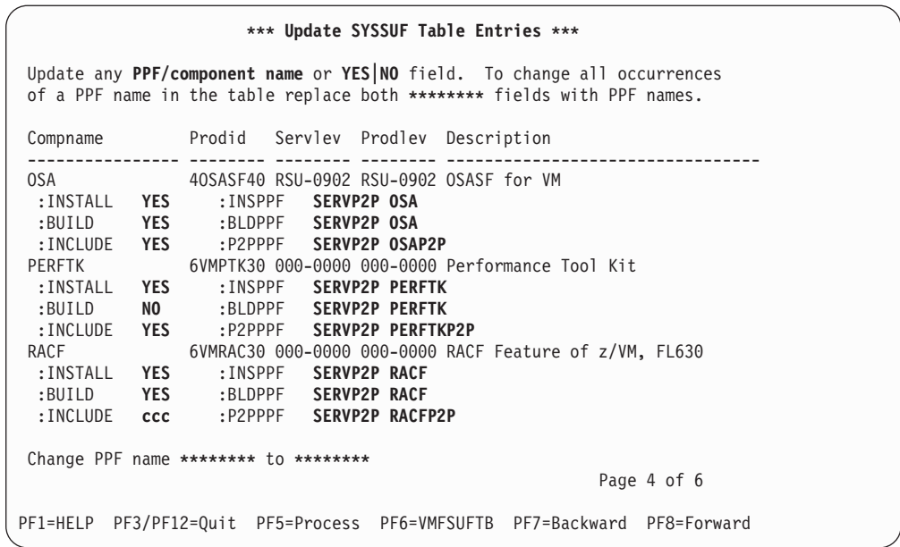
Figure 8. "Update SYSSUF Table Entries" Screen
