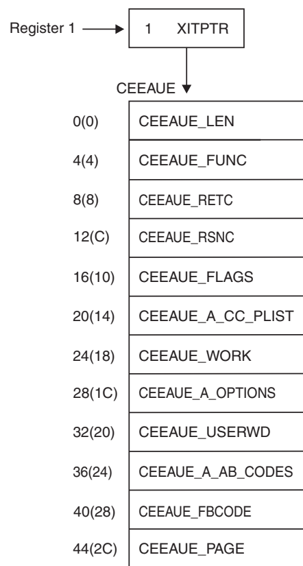
Figure 3. Interface for CEEBXITA Assembler User Exit
