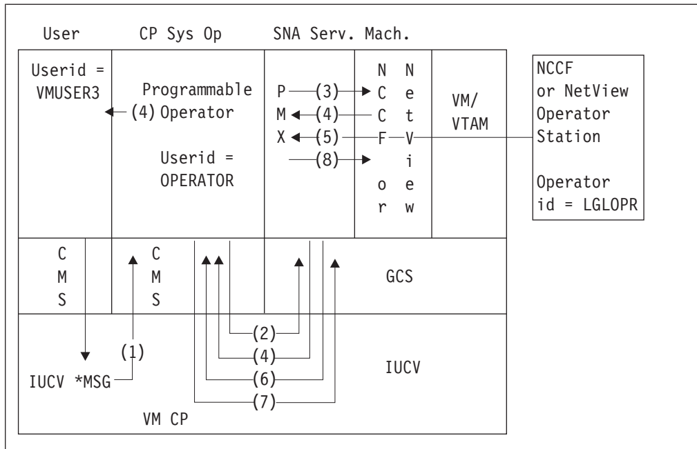
Figure 15. Example of Communication in the Mixed Environment
