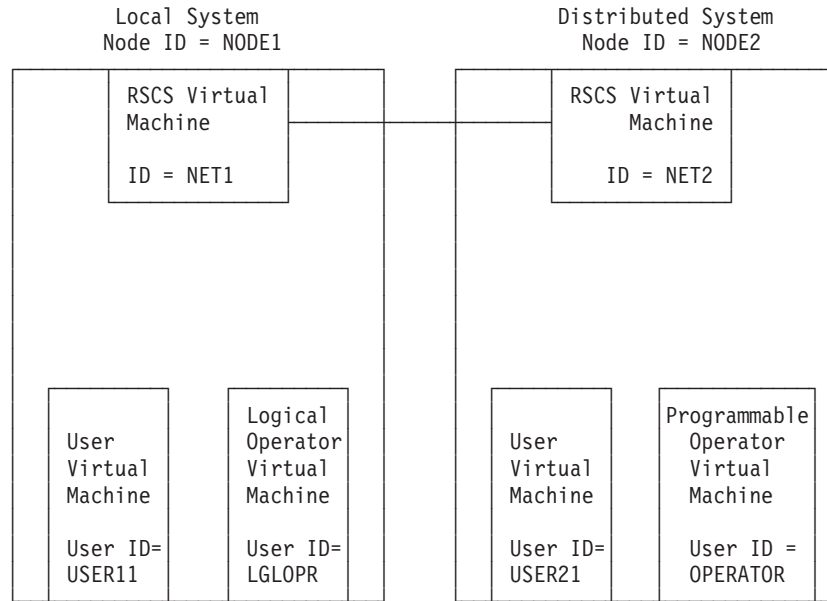
Figure 6. The Programmable Operator Facility in a Distributed System. The logical operator is situated at the host system and the programmable operator is running in a different system at a distributed site.
