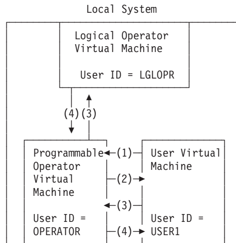
Figure 14. Example of Communication in the Single System Environment
