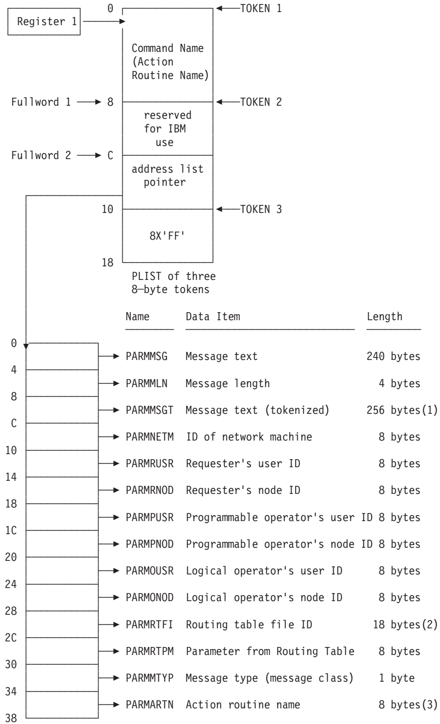
Figure 17. Register Conventions for Invoking an Action Routine
