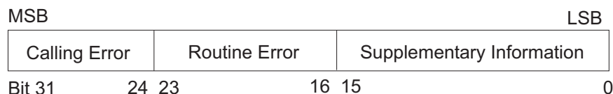
Figure 1. GSS status code bit locations
