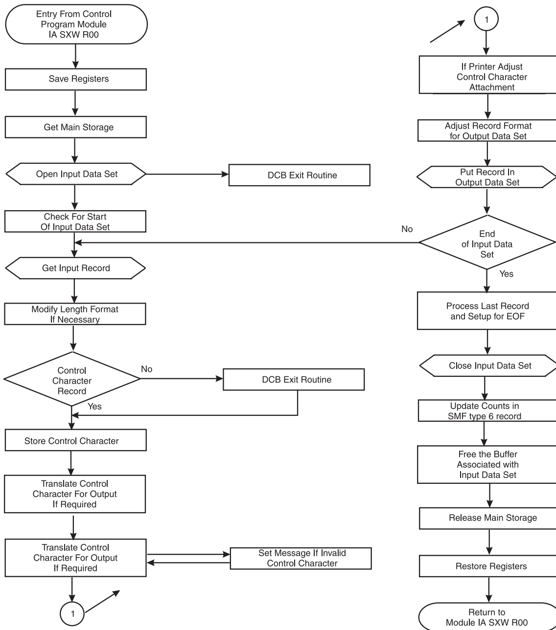
Figure 3. General Flow of IBM's Output Writing Routine
