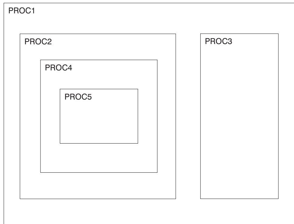
Figure 3. Nested CLISTS
