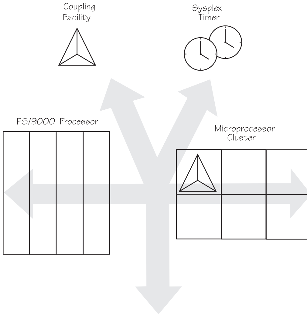
Figure 21. Mixed Processor Sysplex Configuration
