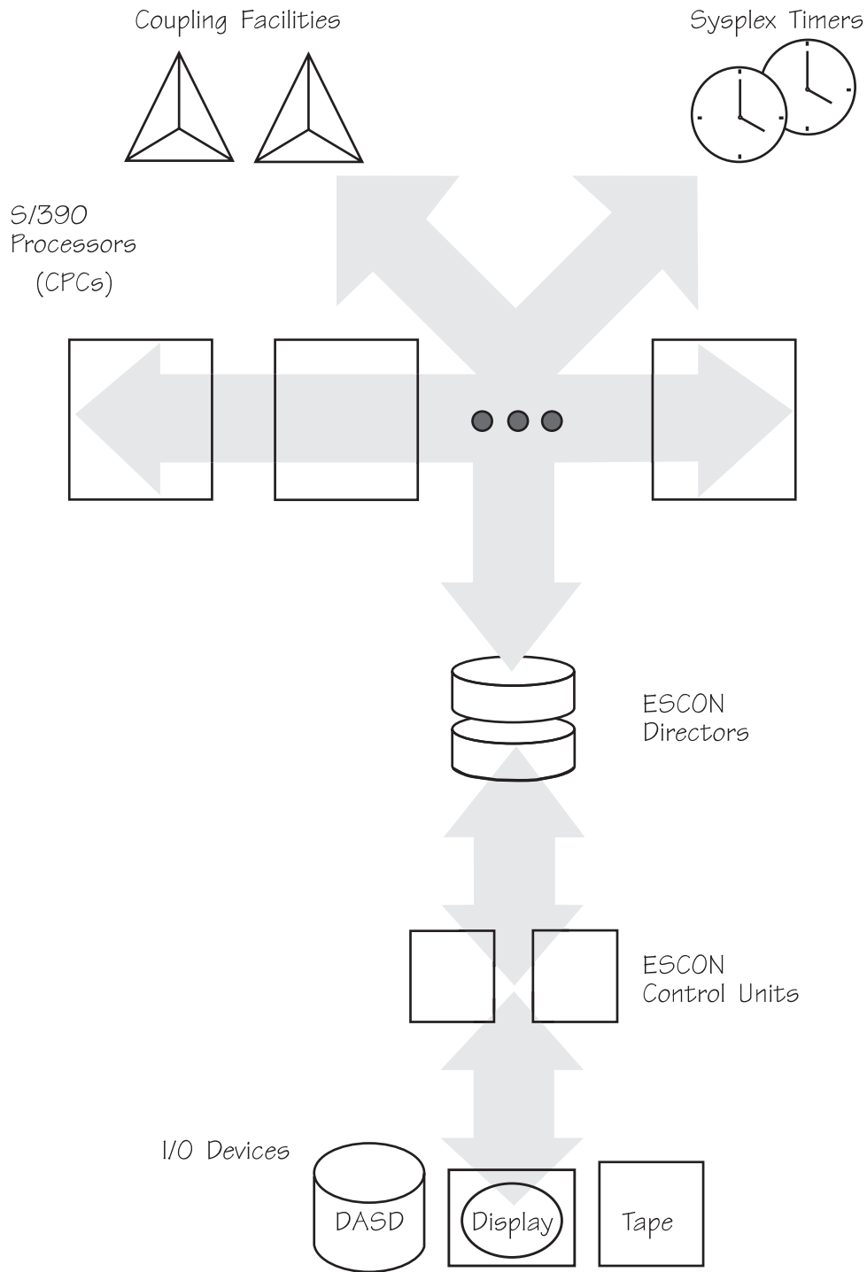
Figure 1. Sysplex Structure
