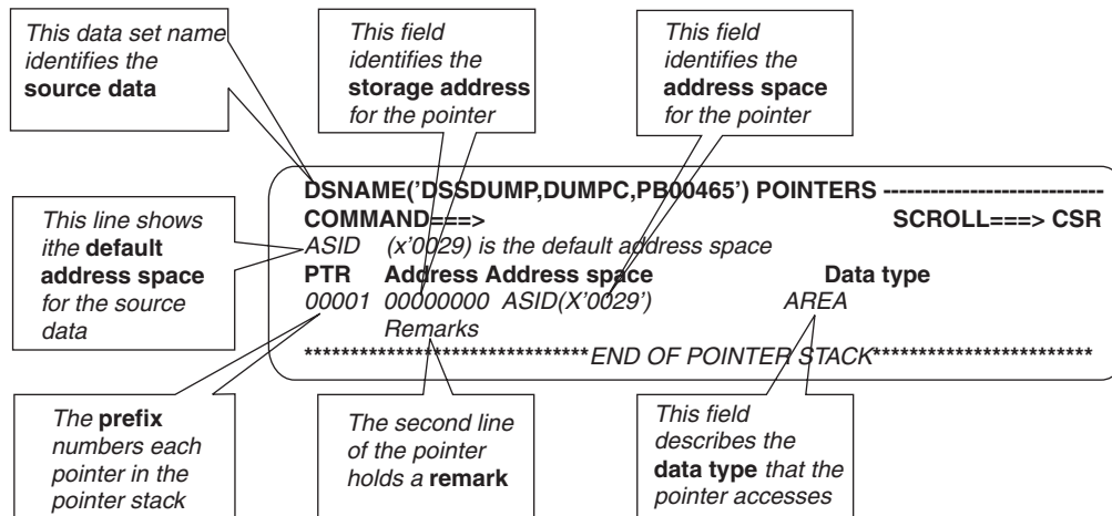
Figure 22. IPCS Dialog Pointer Panel
