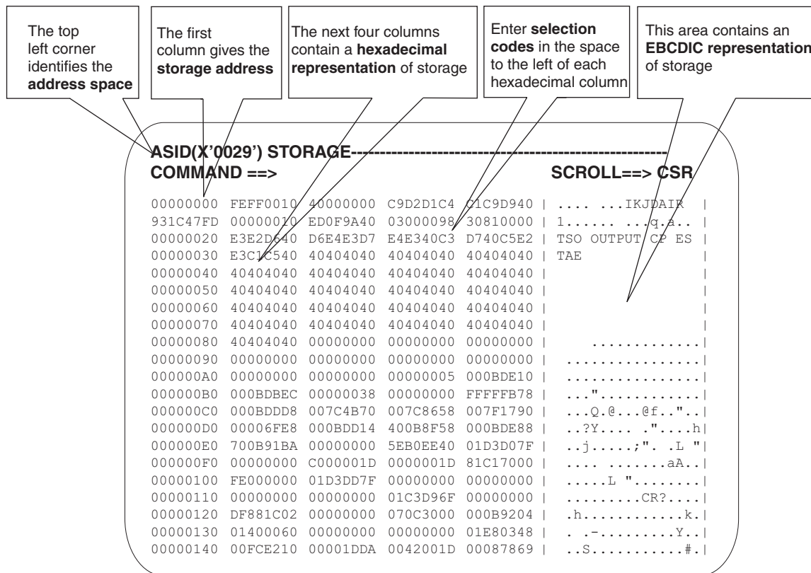
Figure 27. IPCS Storage Panel Browse Option Pointer Panel
