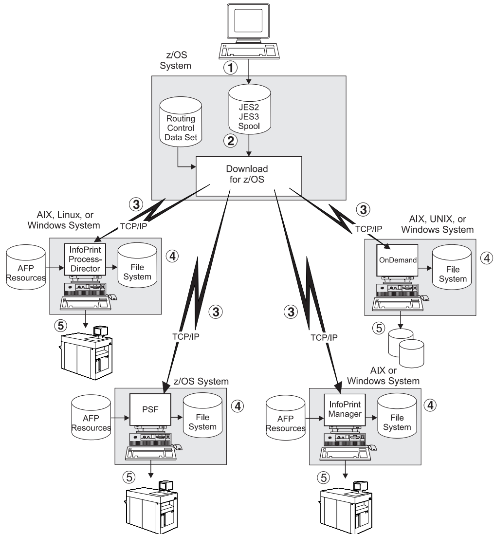
Figure 1. Download for z/OS System Diagram
