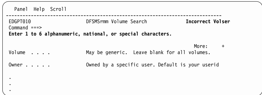
Figure 2. How a Long Message Appears on an ISPF Panel
