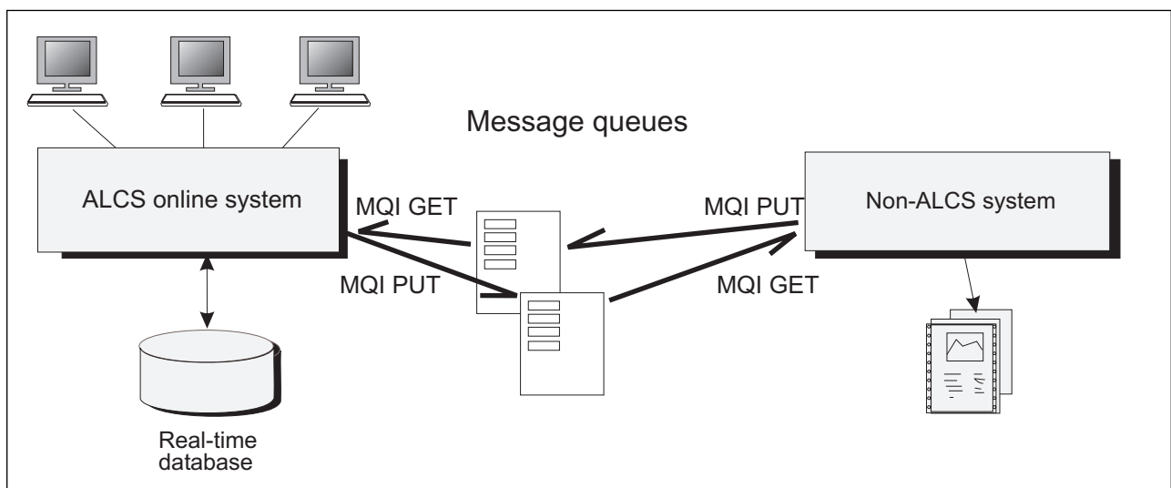
# Figure 4. MQSeries allows ALCS to share data
