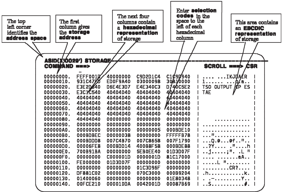
Figure 26. IPCS Storage Panel Browse Option Pointer Panel
