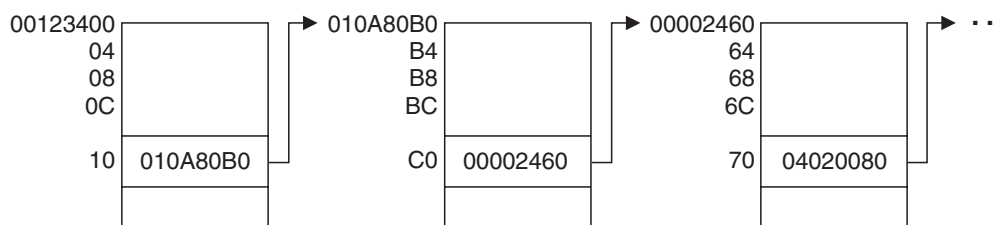
Figure 14. Example of a Chain of Control Blocks
