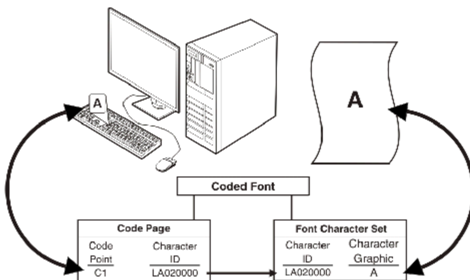
Figure 11: Translation of a keyboard character into a printed character with a code page and FOCA character set
