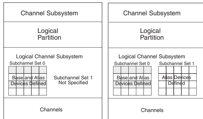
Figure 5. Example of multiple subchannel set configuration
