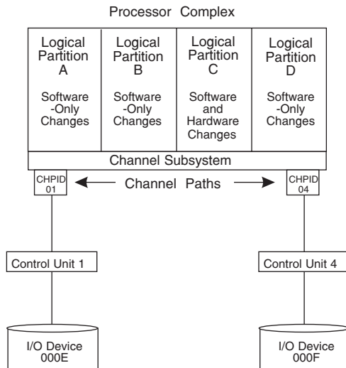
Figure 23. Sample processor running in LPAR mode
