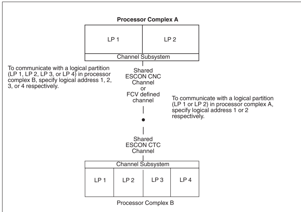
Figure 9. Logical Addresses and Logical Partition Numbers
