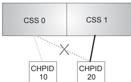
Figure 25. Dynamically adding CHPIDs in a two-LCSS environment on a z990 with compatibility support
