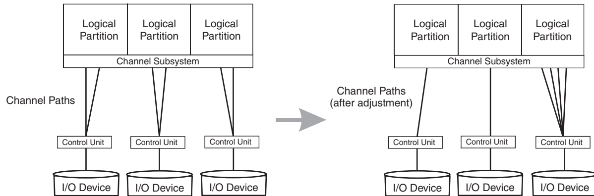
Figure 10. Dynamic Channel Path Management
